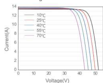
Current-Voltage Curve JAM72S30-540/MR
